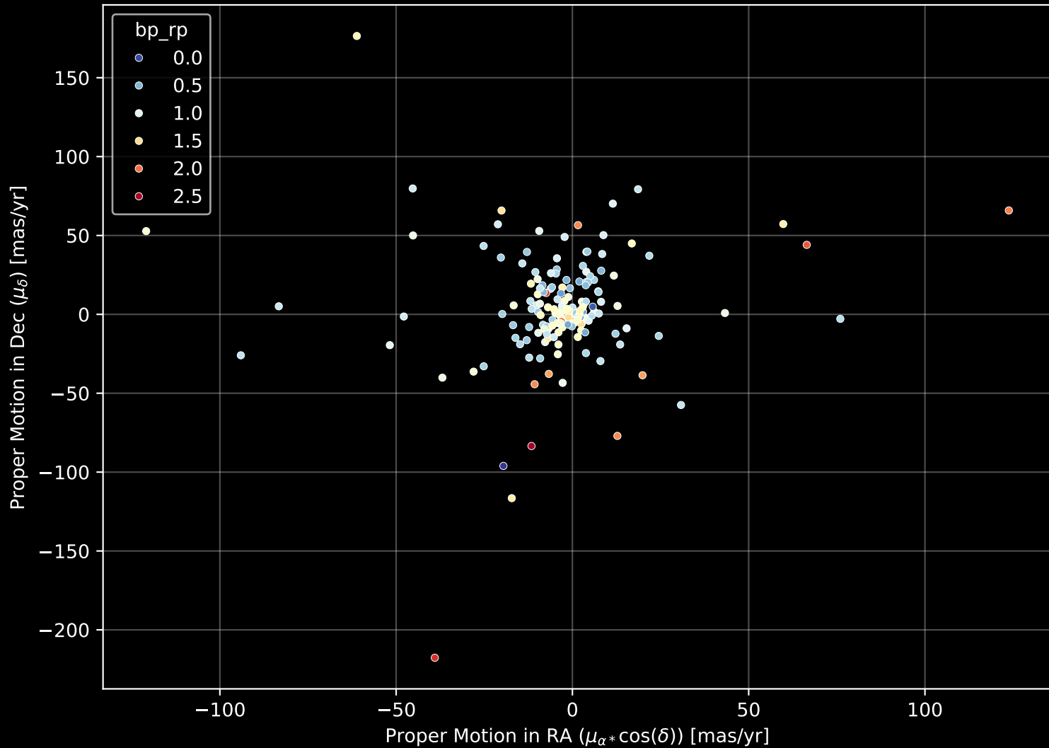
APOGEE DR17 Field: [CVZTILE_100+27_btx] Proper Motion Diagram (n= 170)
