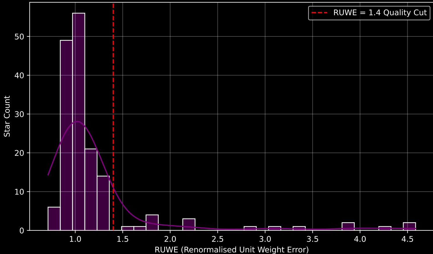
GAPOGEE DR17 Field [CVZTILE_100+27_btx] RUWE Distribution (n= 163)
