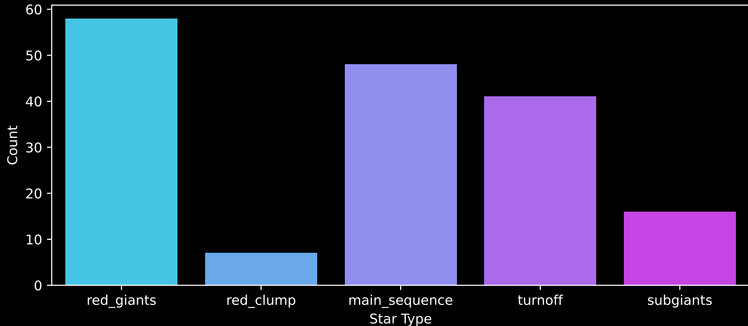
APOGEE DR17 Field: [CVZTILE_100+27_btx] Count plot of Star Type
