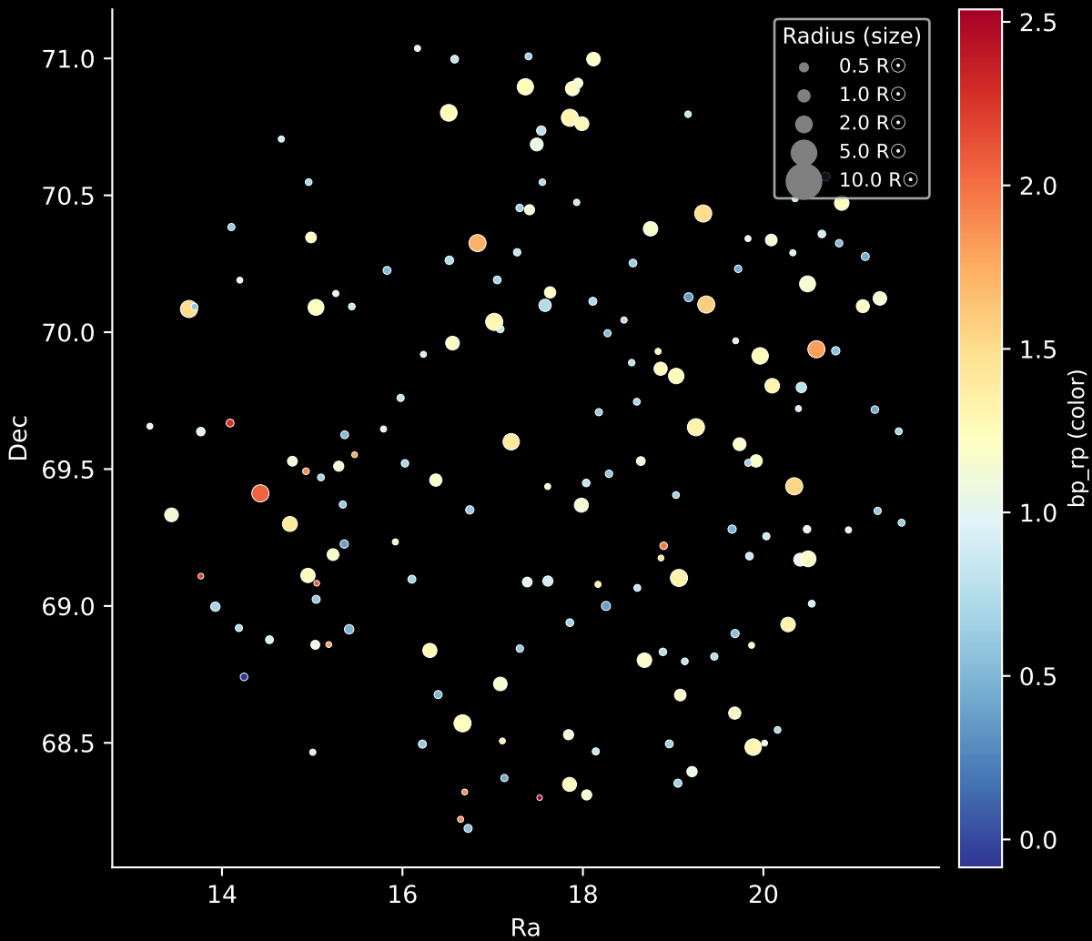
APOGEE DR17 Field: [CVZTILE_100+27_btx] Stars: 170
