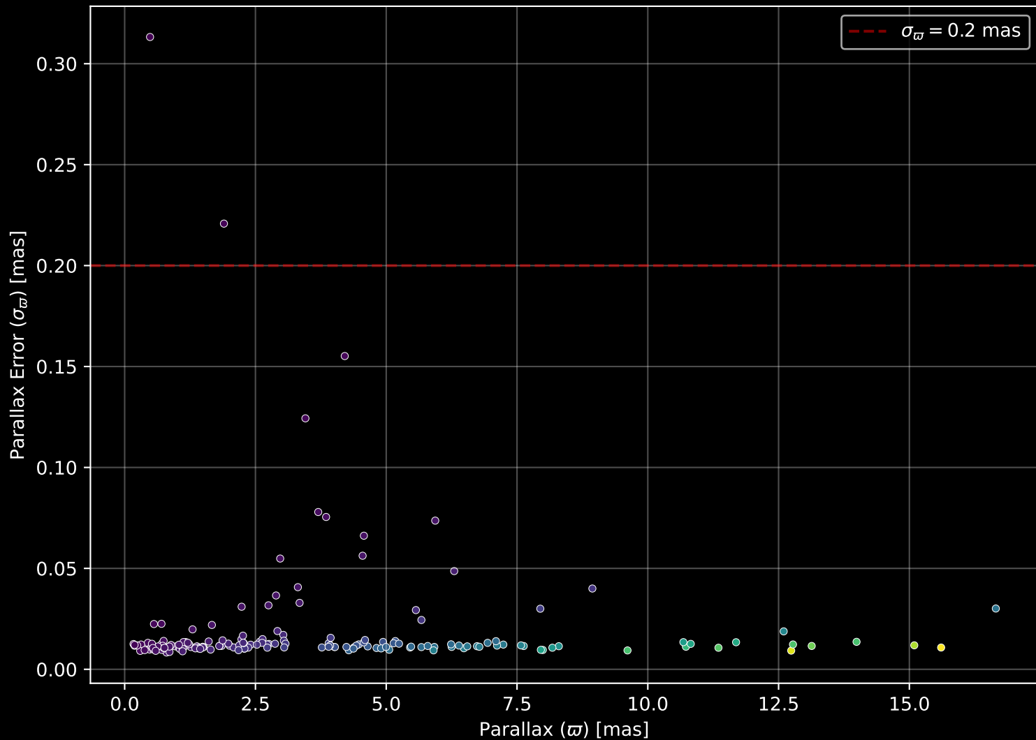
APOGEE DR17 Field: [CVZTILE_100+27_btx] Parallax Quality (n= 170)
