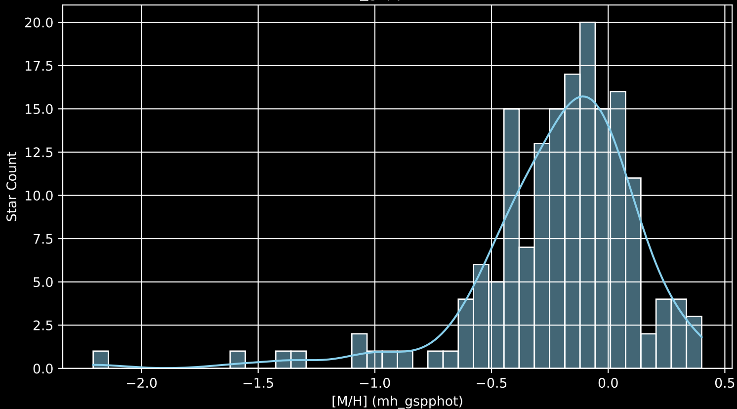
APOGEE DR17 Field: [CVZTILE_100+27_btx [M/H] (mh_gspphot) (n= 168)
